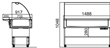
KORO 4/1 SERVICE Refrigerato - Cold - Refrigeré - Kalt - Refrigerado
